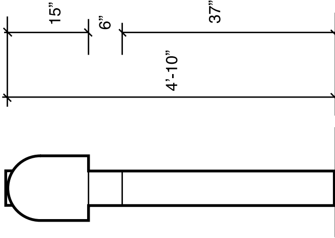
SIDE ELEVATION
